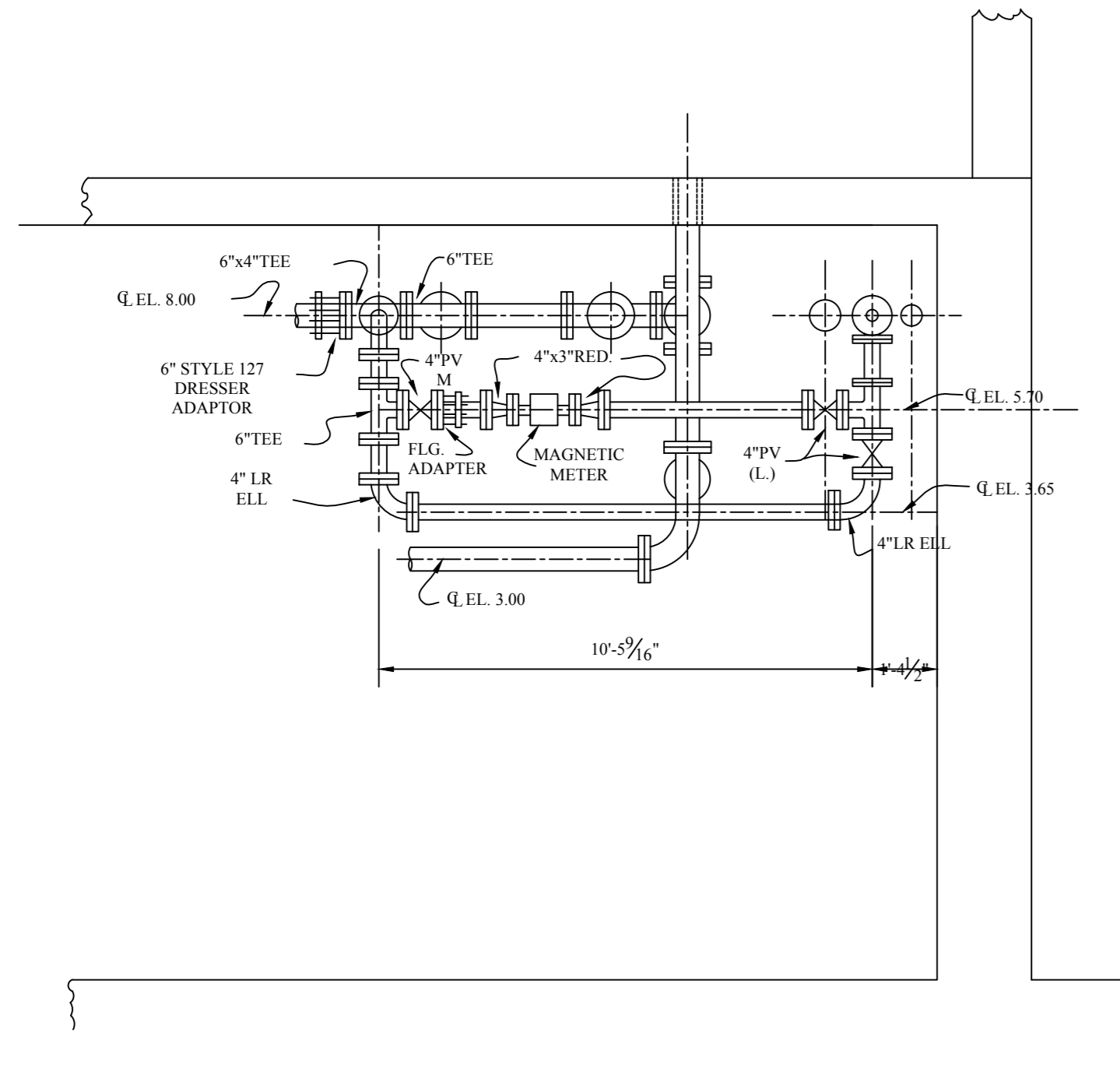
SECTION D 1/4" = 1'-0"
